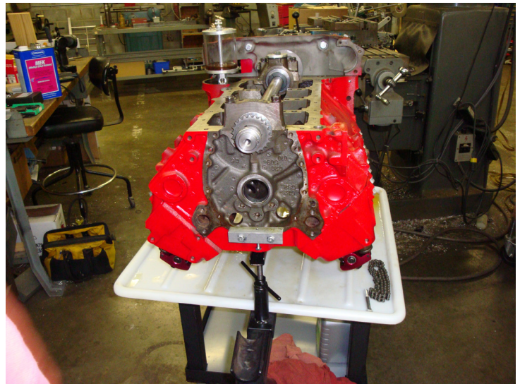
figure 1 - Modified, Inverted Chevrolet 350
