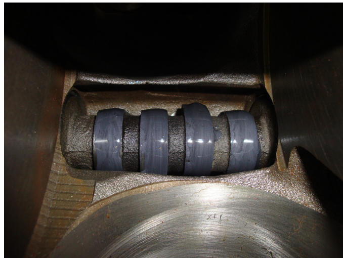
figure 5 - Lubricant #2 on Cam Lobes #7 & #8
